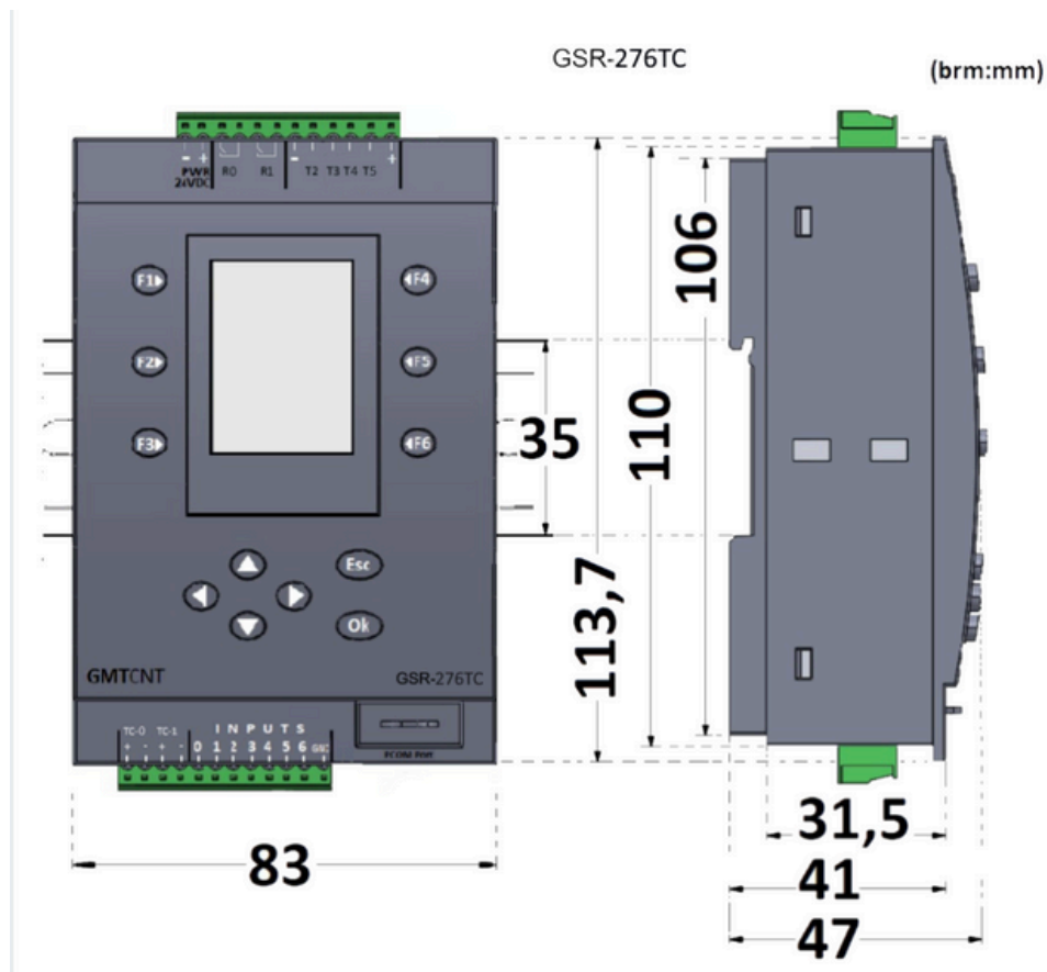
Figure 2: Mechanical Dimensions
