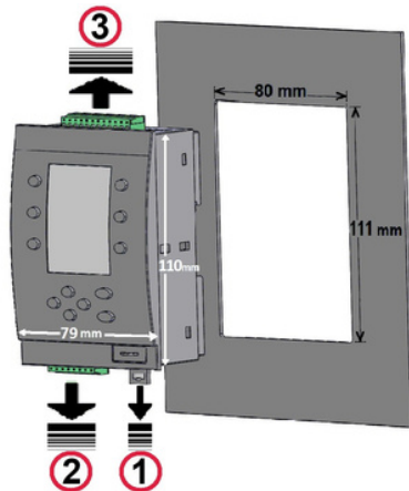
Figure - 4 GSR-T Panel Mounting
