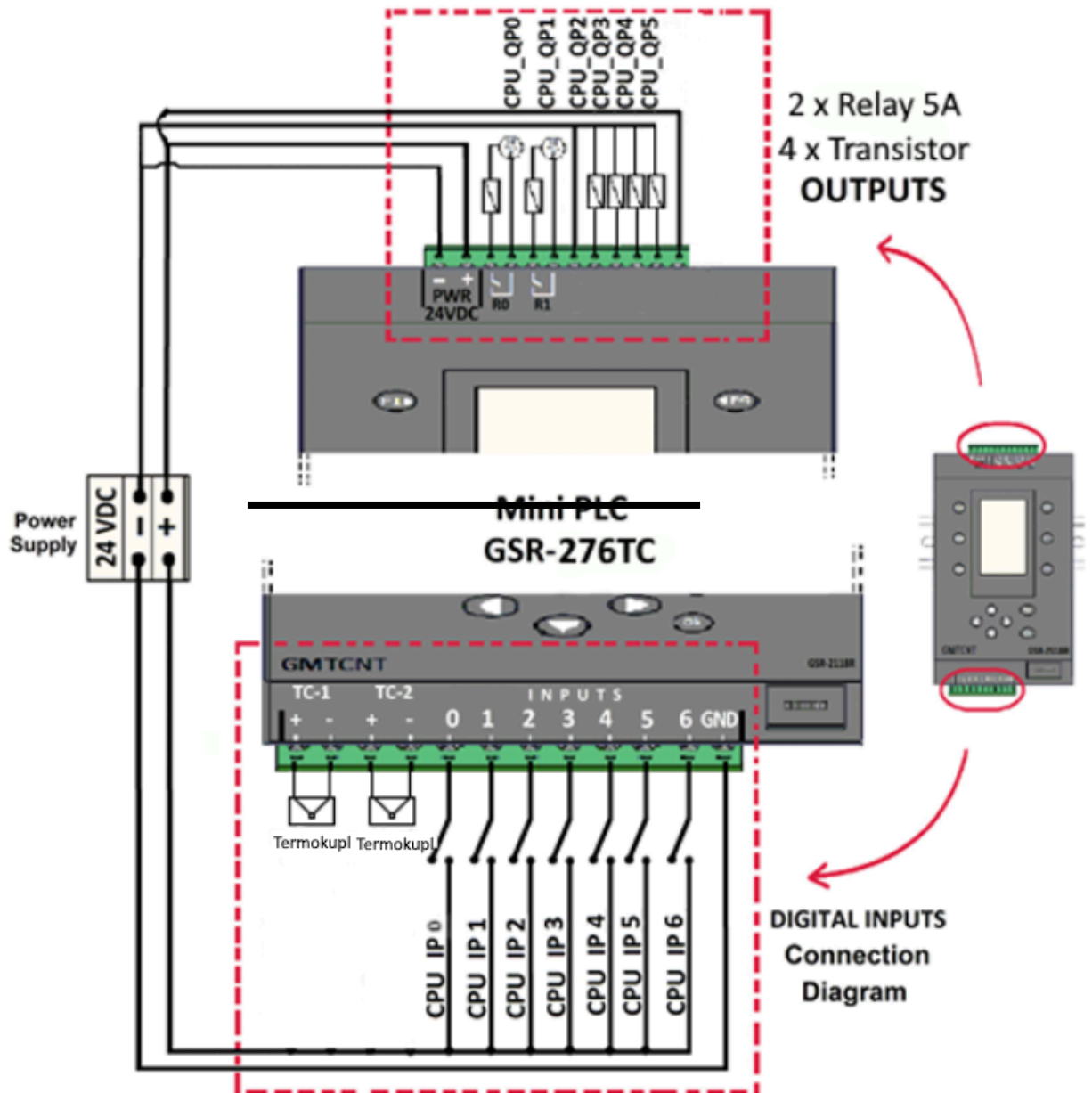
Figure - 11a Digital Input Connectivity Diagram
