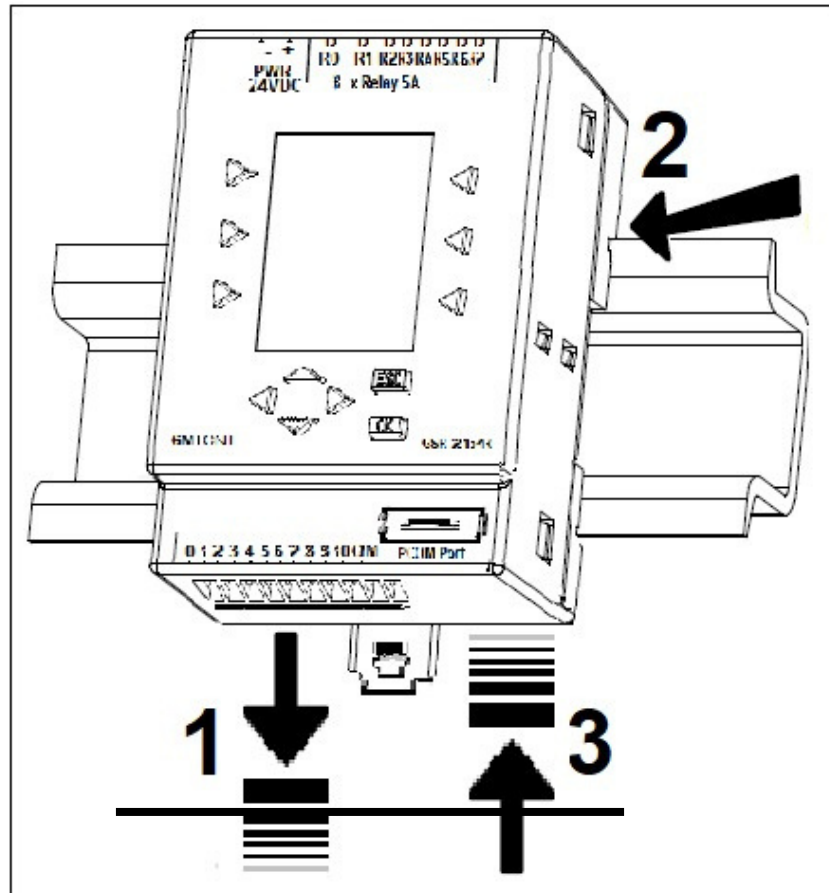
Figure-3 GSR-T DIN Rail Mounting
