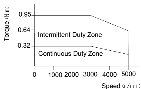
The curve of torque-speed
