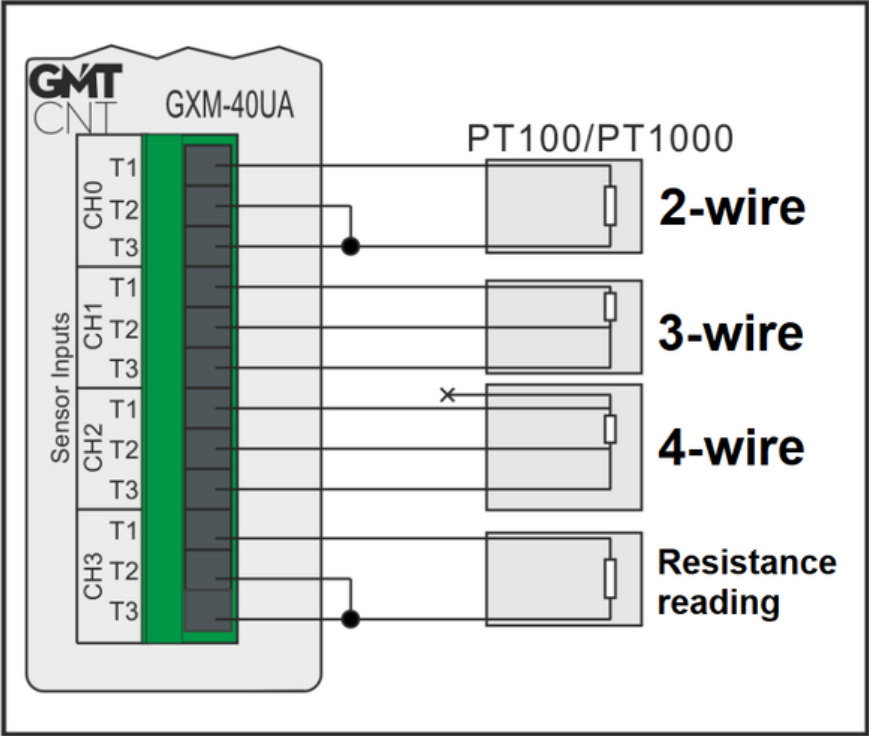
PT100, PT1000 and Resistance Connections
