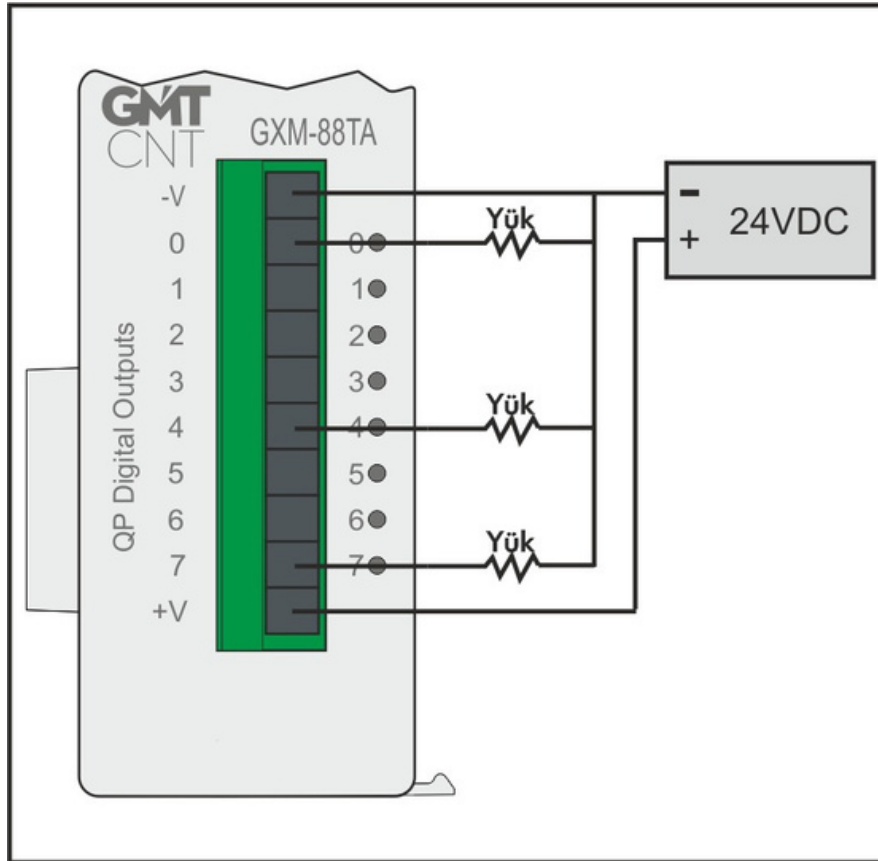
DO, Transistor output connection diagram
