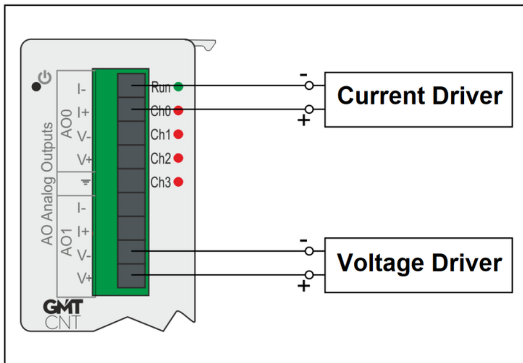
Analog Output Connection Diagram
