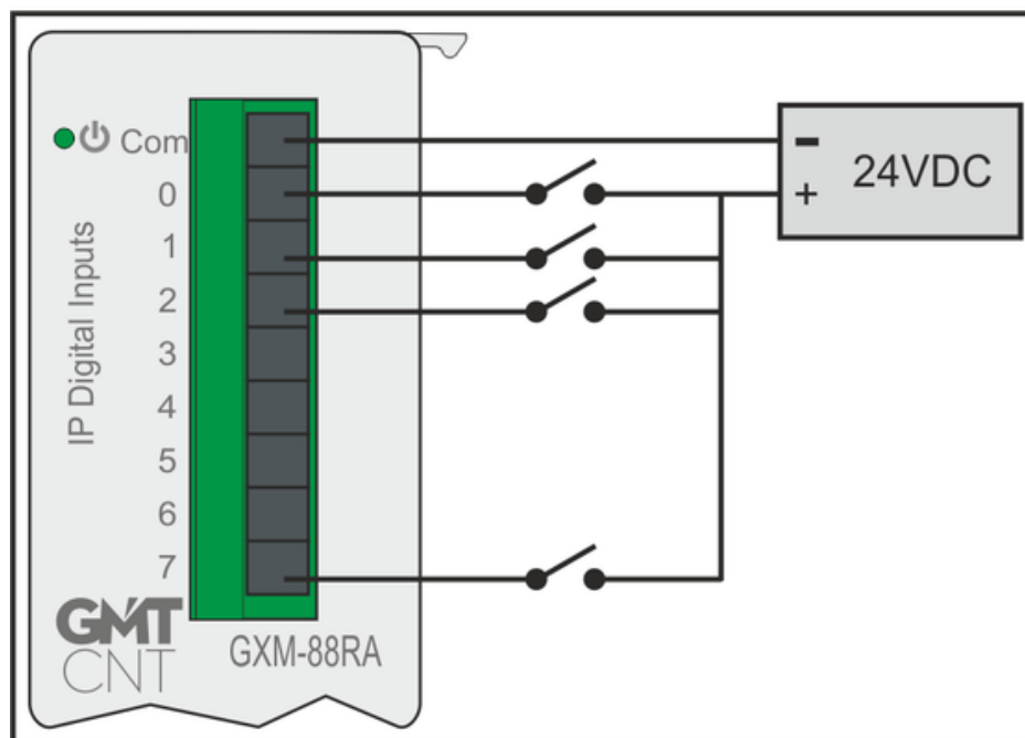
DI, PNP type connection diagram
