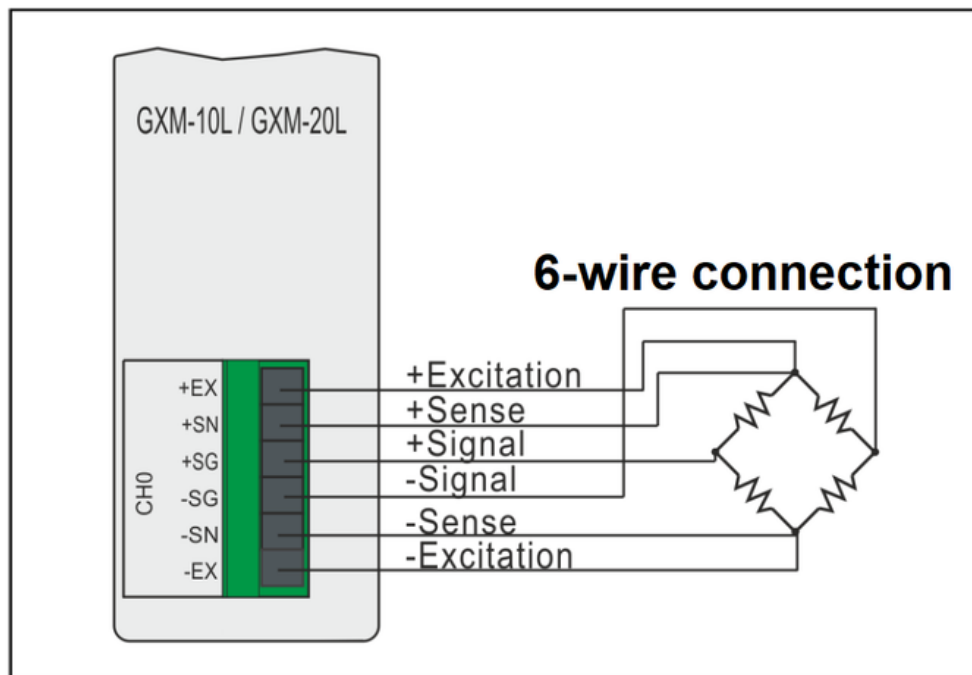
6-Wired Load Cell Connection
