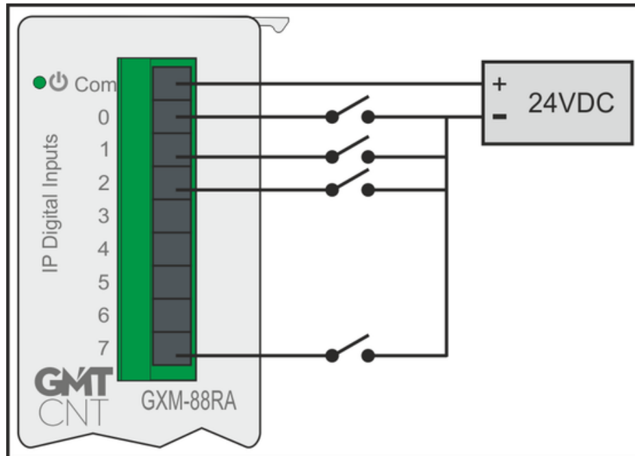
DI, NPN type connection diagram
