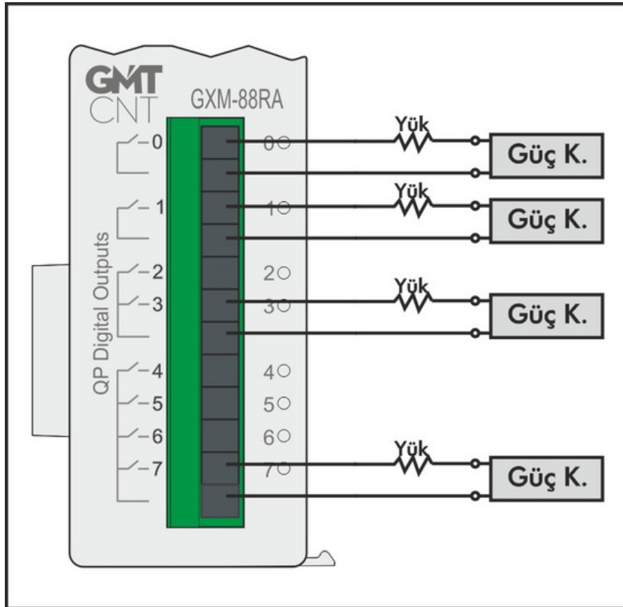
DO, Relay output connection diagram
