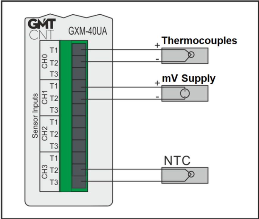
Thermocouple, NTC and mV Connections
