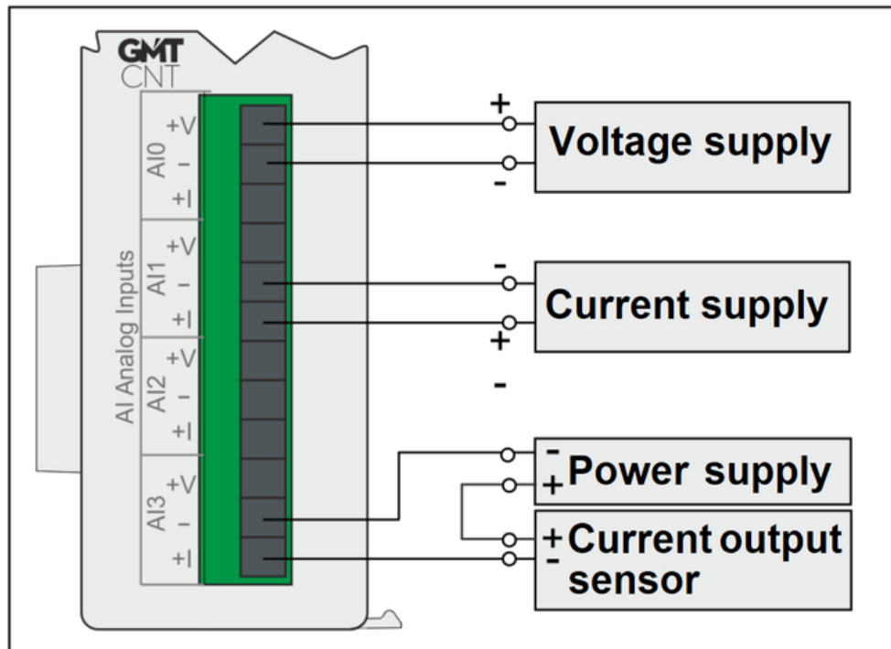
Analog Input Connection Diagram
