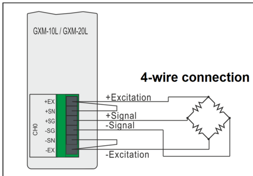
4-Wired Load Cell Connection
